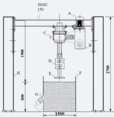
Fig. 4. Cross-sectional view of the loading frame.
